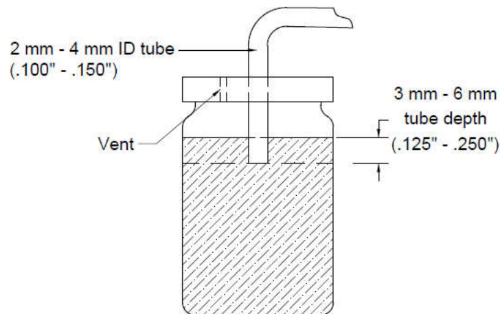
Figure 1—Volumetric Device
